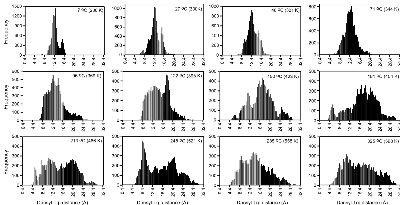
FIGURE 9 Distributions of dansyl-Trp distances for DansMsp1capC at various temperatures calculated from the REMD data over simulation time 2–3 ns (10,000 coordinate sets per temperature). Bars are drawn for 0.2-Å intervals. Distance, x axis; number of occurrences of distance, y axis.
